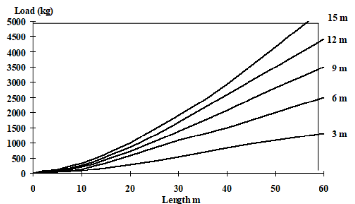
Tensile load in cables suspended in a steel silo
