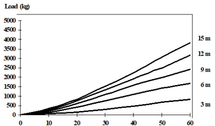
Tensile load in cables suspended in a concrete silo
