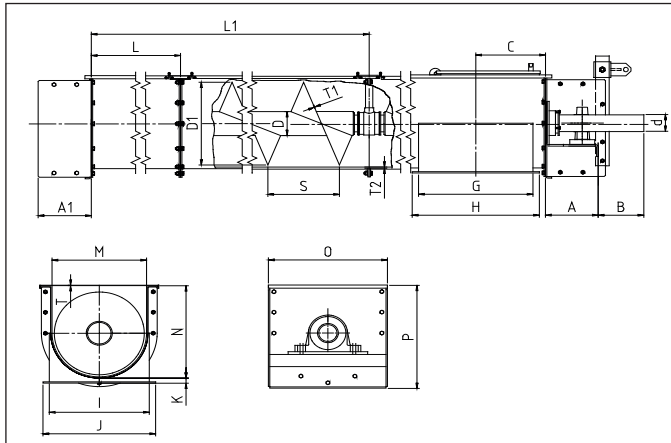
Conveyor type SUH - DIMENSIONS
