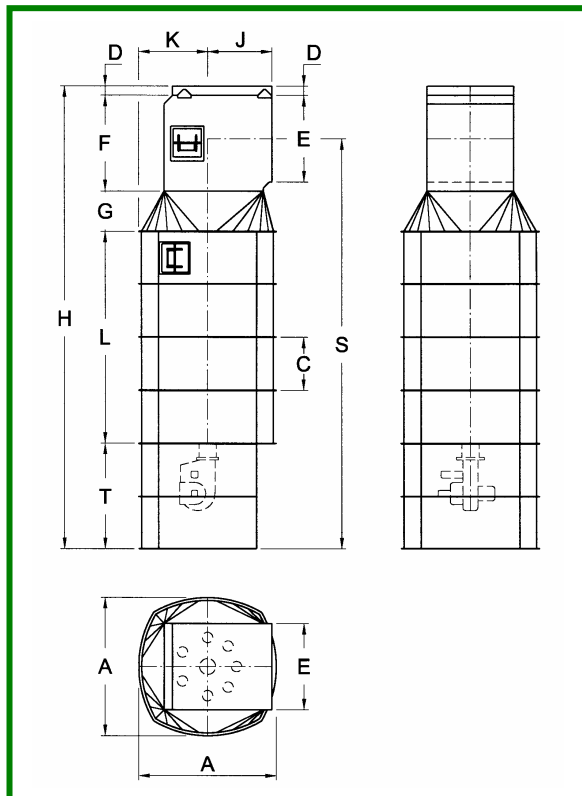
Figure 1: Vertical VD furnace
