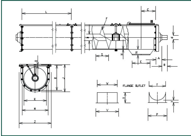
Conveyor type SUH - DIMENSIONS
